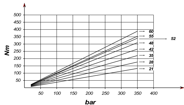
DRIVE TORQUE
