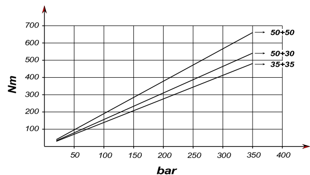
DRIVE TORQUE
